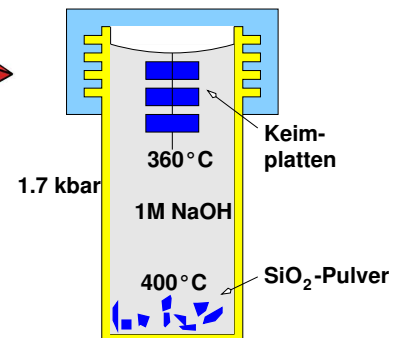
Hydrothermale Quarzsynthese
